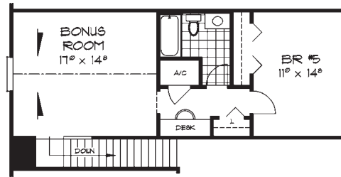
BONUS ROOM "B"
