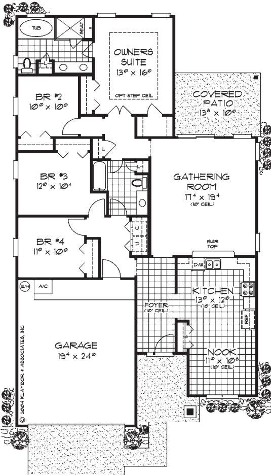
"DAVENPORT" 1806 SQ FT (LIVING) 40' x 68'
