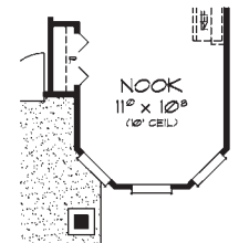
OPTION #5 BAY AT NOOK -9 SQ FT (LIVING)
