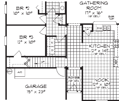
FIRST FLOOR W/ BONUS ROOM
