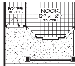
OPTION #3 BAY AT NOOK
