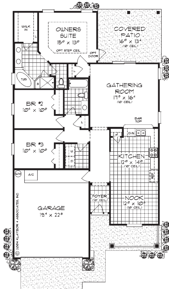
"HAMILTON" 1591 SQ. FT. (LIVING) 38' x 64'
