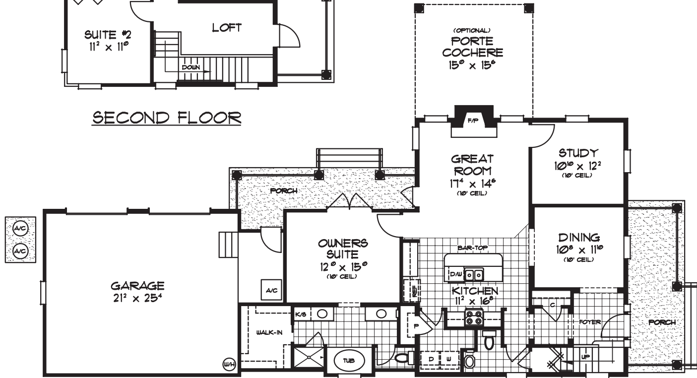
FIRST FLOOR
