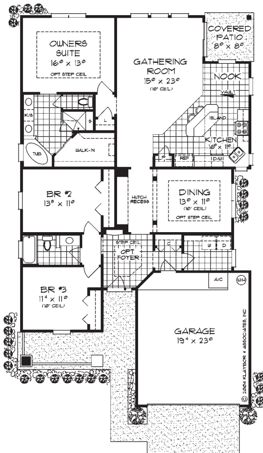
"OMAHA" 1839 SQ. FT. (LIVING) 40' x 68'
