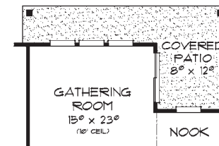
OPTION #4 +4' OF DEPTH TO COVERED PATIO +4' TO DEPTH OF HOUSE
