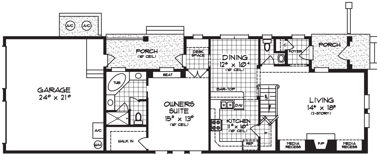
FIRST FLOOR
